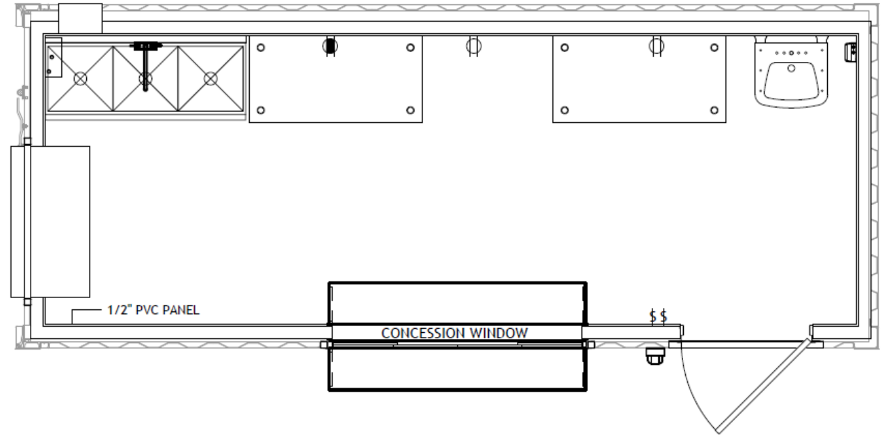
ARCHITECTURAL FLOORPLAN
