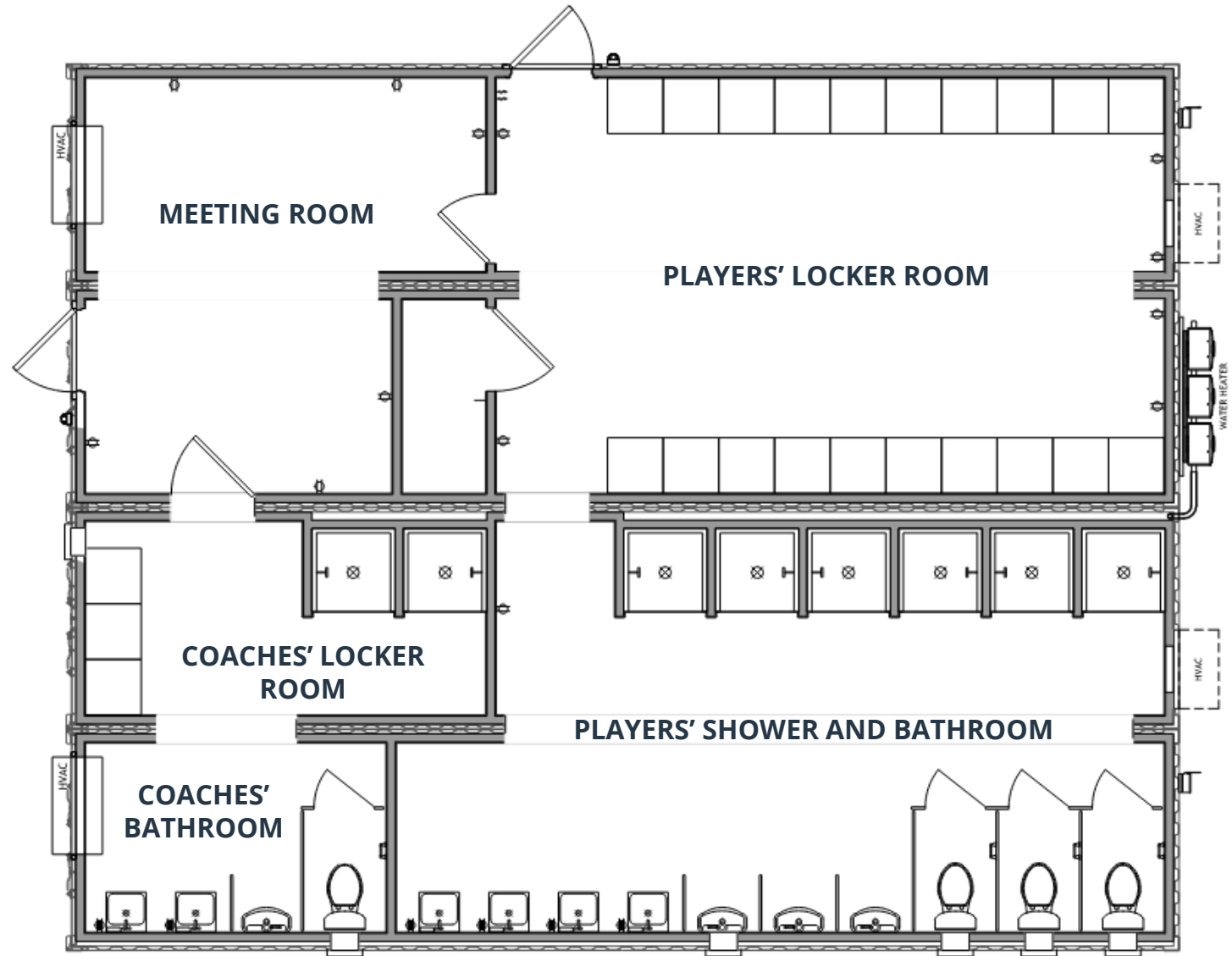
ARCHITECTURAL FLOORPLAN
