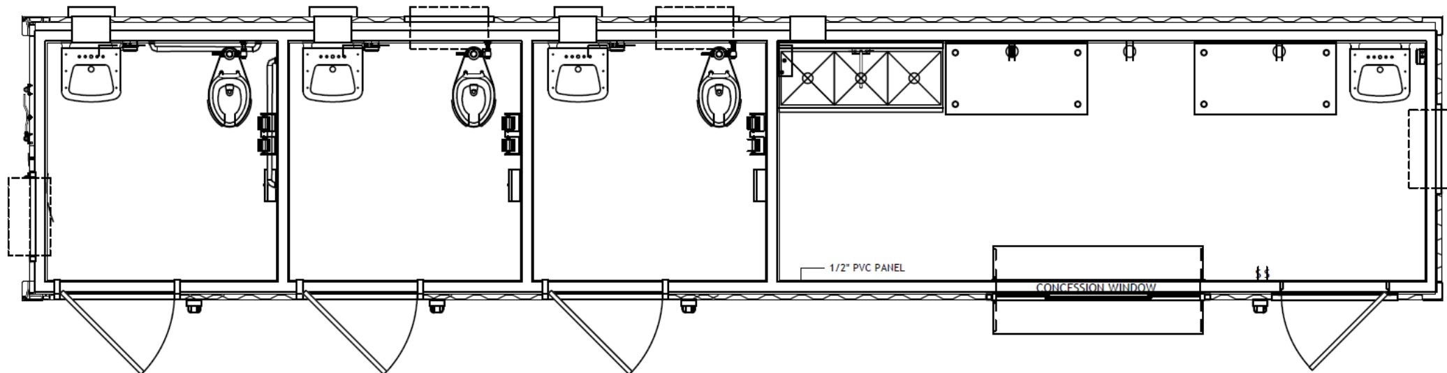
ARCHITECTURAL FLOORPLAN
