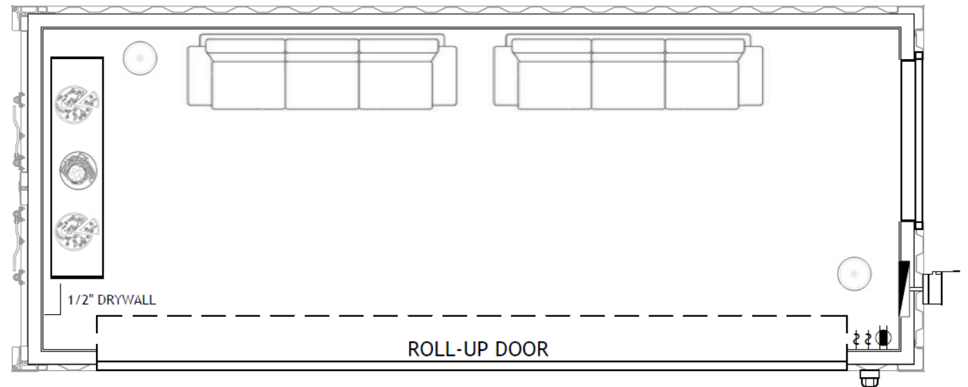
ARCHITECTURAL FLOORPLAN
