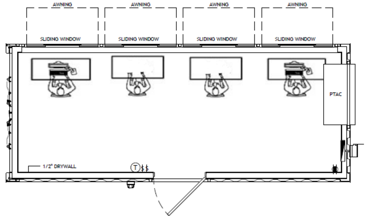
ARCHITECTURAL FLOORPLAN
