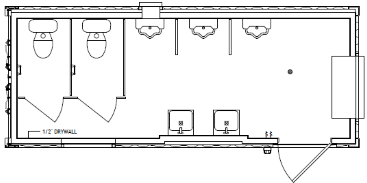
ARCHITECTURAL FLOORPLAN
