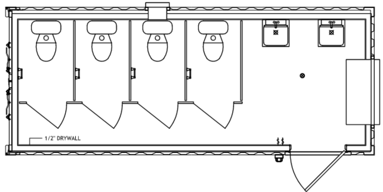
ARCHITECTURAL FLOORPLAN
