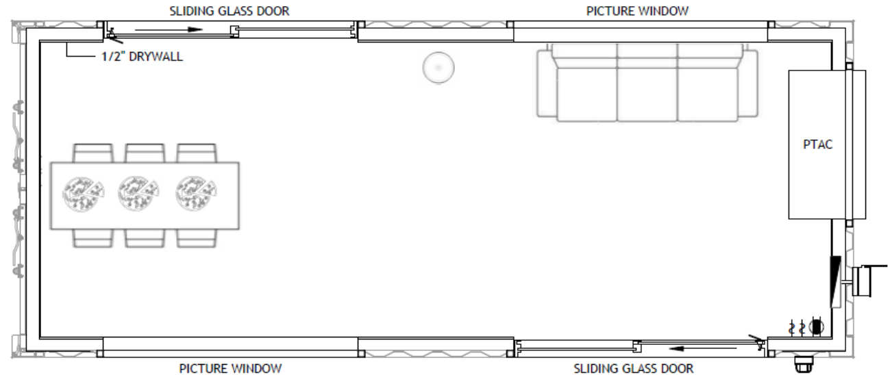
ARCHITECTURAL FLOORPLAN
